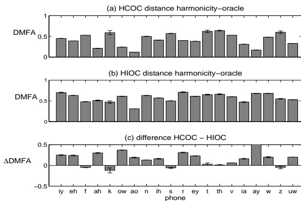
Figure 6. Barchart of the difference DMFA between the MFA 's of oracle and harmony masks for the (a) HCOC subset, (b) the HIOC subset, and (c) the difference \Delta DMFA between the two subsets. The distance function only considered a set of frequencies estimated to be the most important for recognition, using Eq. 6.
