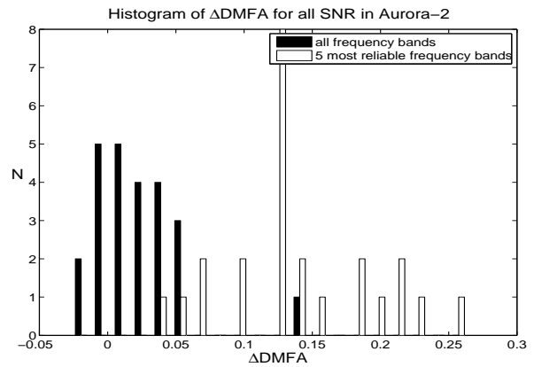
Figure 3. A histogram with phone averaged \Delta DMFA values obtained by analyzing testset A of the AURORA-2 corpus. The corpus was divided in 4 noise types for every SNR. SNR values were 20, 15, 10, 5, 0, -5 dB. This resulted in 24 analysis tasks. The y -axis shows the number N of analysis tasks resulting in a certain \Delta DMFA
