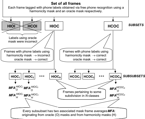
Figure 1. The hierarchy of sets, subsets and subsubsets resulting in mask frame averages.
