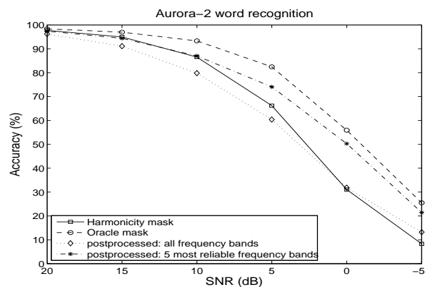
Figure 7. Word recognition results. Recognition results were obtained using the oracle mask, the harmony mask, the post-processed harmony mask using all frequency bands and the post-processed harmony mask using the 5 frequency bands estimated to be crucial for recognition.
