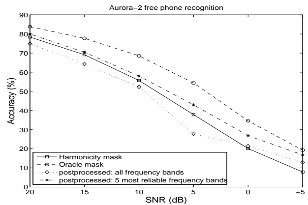
Figure 5. Phone recognition results. Recognition results were obtained using the oracle mask, the harmony mask, the post-processed harmony mask using all frequency bands and the post-processed harmony mask using the 5 frequency bands estimated to be crucial for recognition.
