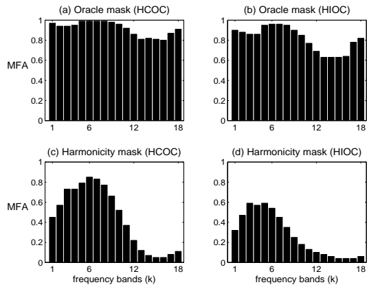
Figure 2. Example. The Mask Frame Average ( MFA ) of frames in the HCOC subset (a) and (c), and the HIOC subset (b) and (d). The sound class used to select the subset was the phone label /ah/ . The MFA shows for every frequency band the fraction of frames that were considered reliable
