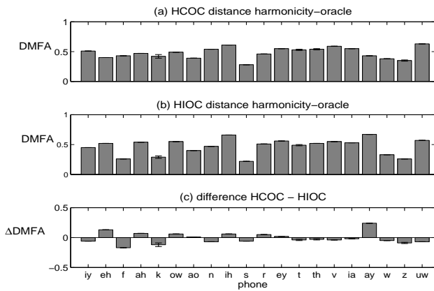
Figure 4. Barchart of the difference DMFA between the MFA 's of oracle and harmony masks for the (a) HCOC subset, (b) the HIOC subset, and (c) the difference \Delta DMFA between the two subsets. The distance function took all frequency bands into account with equal weight, using Eq. 5.
